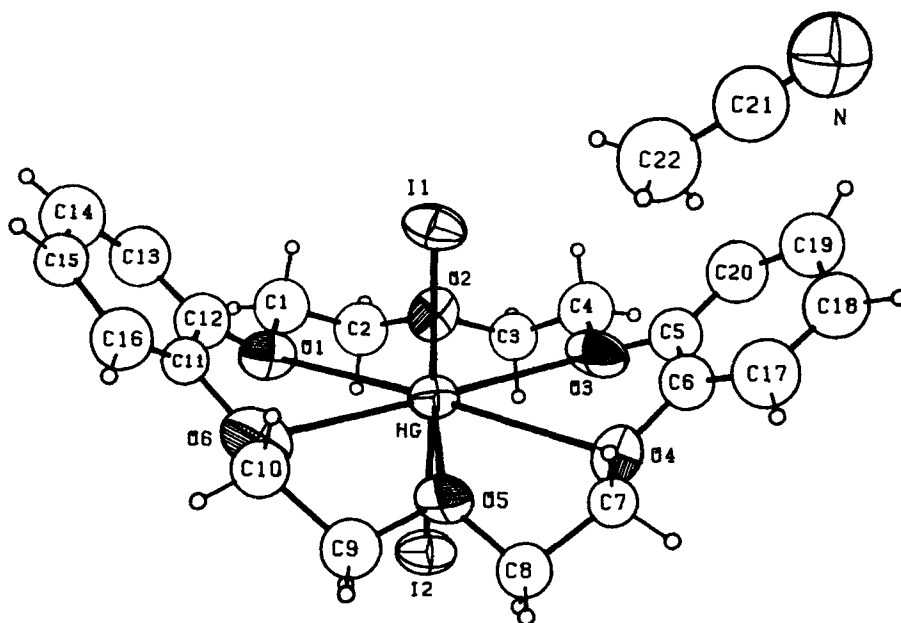
Figure 2 [\text{HgI}_2(\text{dibenzo-18-crown-6})]\cdot\text{CH}_3\text{CN} .
