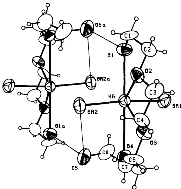
Figure 5 [\text{HgBr}_2(\text{EO4})] . The Hg-Br(2) a distance is long (4.157(2)Å) but in a geometrically significant position. The dimeric unit shown resides around a crystallographic centre of inversion. The symmetry code 'a' refers to \bar{x} , 1-y, 1-z.
